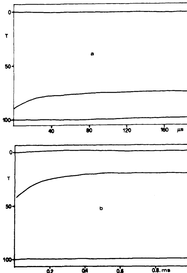
Figure 3. Oscilloscope traces showing the "instantaneous" and the "slow" parts of the grow-in of the absorption at 370 nm after laser excitation of azide 1a (not absorbing at this wavelength): a, in acetonitrile; b, in cyclohexane.
