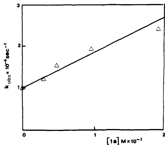
Figure 5. Rate constants for quenching of benzophenone triplet (monitored at 532 nm) at increasing 1a concentrations.
