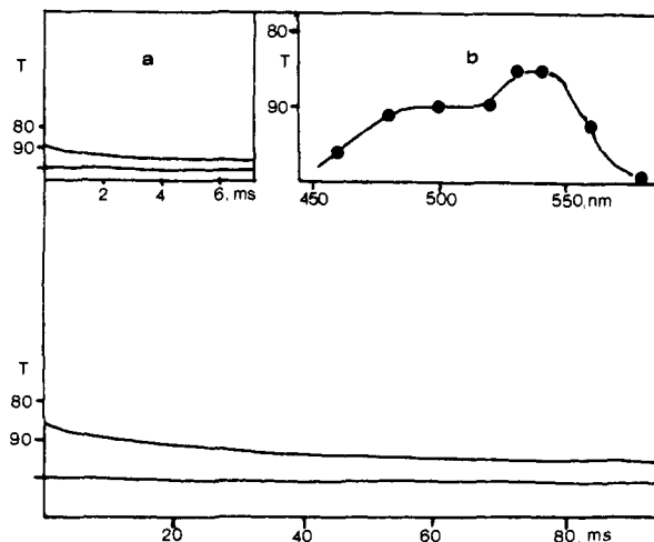
Figure 4. Oscilloscope traces showing the transient absorption at 490 nm after flashing a solution of heteropentalene 2c in cyclohexane. Inset a, transient absorption observed at 530 nm after flashing a solution of acetophenone ( 1.35 \times 10^{-2} \text{ M} ) and azide 1a ( 2 \times 10^{-3} \text{ M} ) in acetonitrile. Inset b, absorbance spectrum observed 5 ms after flash under the same conditions as in the previous experiment.
