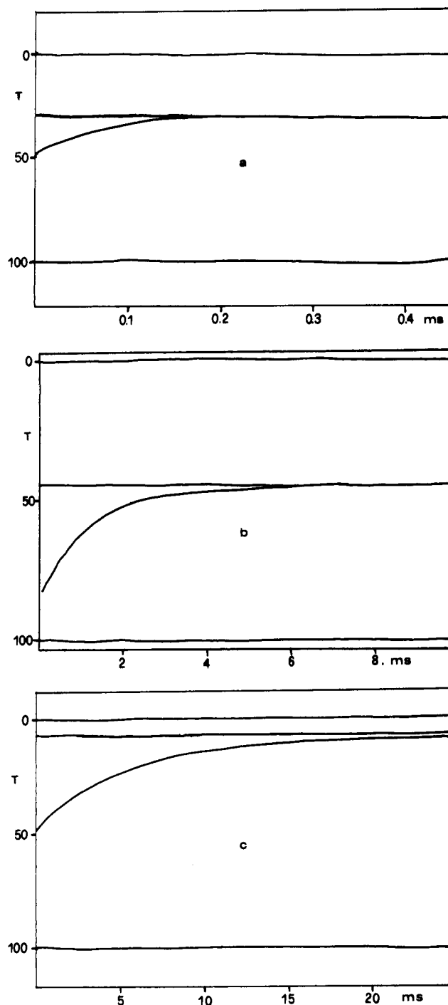
Figure 2. Oscilloscope traces showing the reversible bleaching (measured at 370 nm): a, heteropentalene 2a in acetonitrile; b, the same in cyclohexane; c, heteropentalene 2c in acetonitrile. The first trace is obtained by laser flash photolysis, the other ones by conventional lamp discharge flash photolysis (see the Experimental Section).
