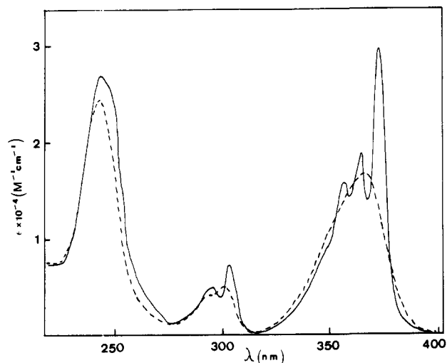
Figure 1. Absorption spectra of compound 2c in cyclohexane (—) and in acetonitrile (---).
